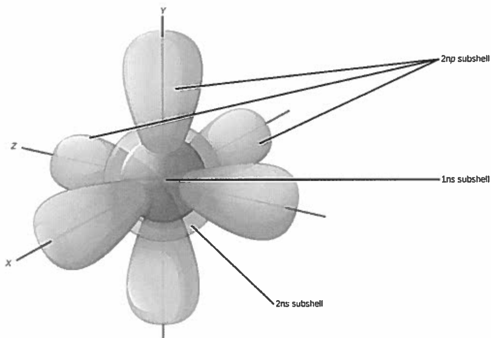
Figure 2.8 The s subshells are shaped like spheres. Both the 1 n and 2 n principal shells have an s orbital, but the size of the sphere is larger in the 2 n orbital. Each sphere is a single orbital. p subshells are made up of three dumbbell-shaped orbitals. Principal shell 2 n has a p subshell, but shell 1 does not.
