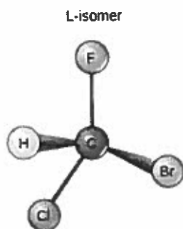
Figure 2.24 Molecules that have the same number and type of atoms arranged differently are called isomers. (a) Structural isomers have a different covalent arrangement of atoms. (b) Geometric isomers have a different arrangement of atoms around a double bond. (c) Enantiomers are mirror images of each other.
