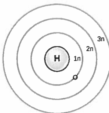
Figure 2.6 The Bohr model was developed by Niels Bohrs in 1913. In this model, electrons exist within principal shells. An electron normally exists in the lowest energy shell available, which is the one closest to the nucleus. Energy from a photon of light can bump it up to a higher energy shell, but this situation is unstable, and the electron quickly decays back to the ground state. In the process, a photon of light is released.
